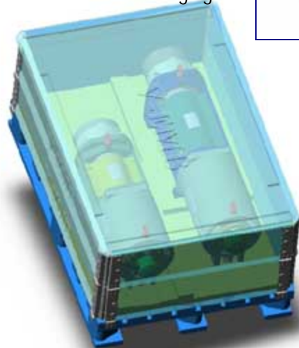
How the part will fit in Volvo Packaging
