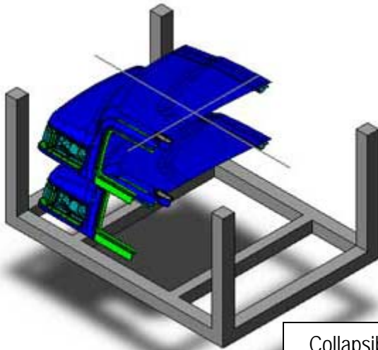
Racks to move truck cabs
